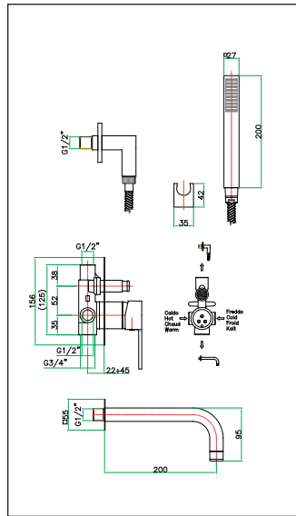
art. 77 CR 7509
