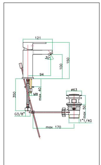
art. 77 CR 7530
