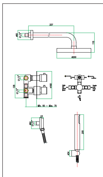
art. 31 CR 0995
