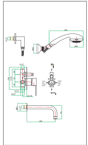
art. 77 CR 7538
