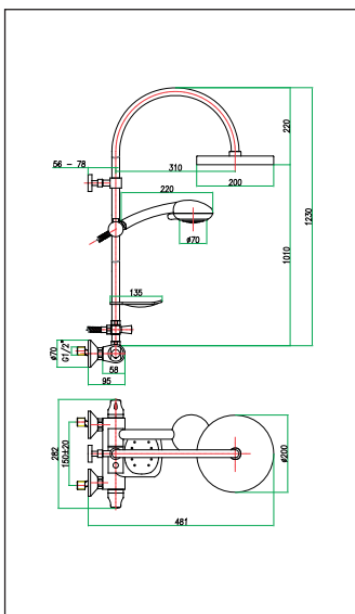
art. 36 CR 0988
