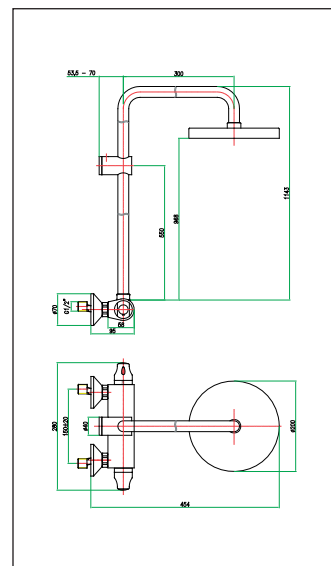
art. 36 CR 0975
