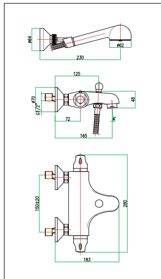
art. 36 CR 0951
