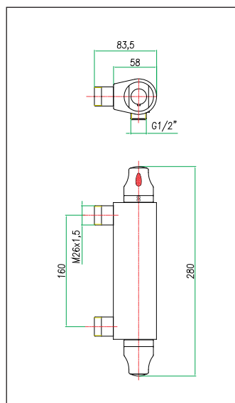
art. 36 CR 0982
