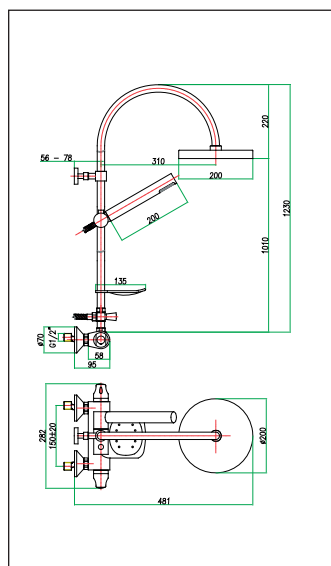
art. 36 CR 0989
