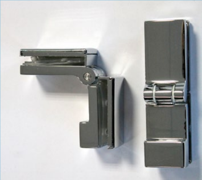
PONZA EVO CERNIERE - HINGES - SCHARNIERE - CHARNIÈRE
